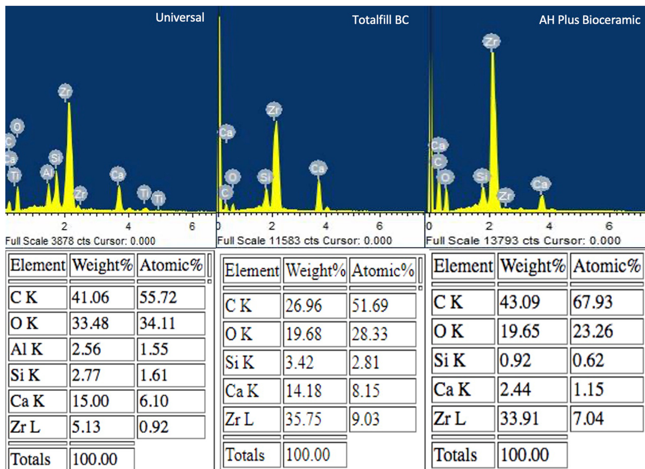
FIGURE 2 – Energy dispersive spectroscopic plots showing the elements present. All materials contained calcium, silicon, oxygen, and zirconium with BC Universal sealer, including titanium and aluminum.
